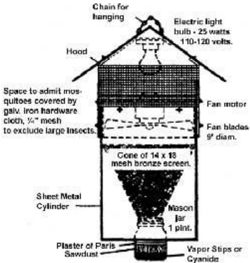
NEW JERSEY - TYPE LIGHT TRAP
